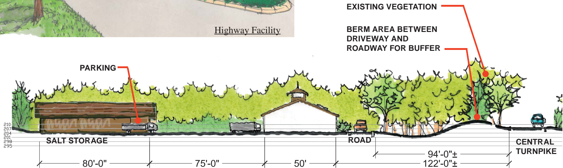
Section From Roadway
